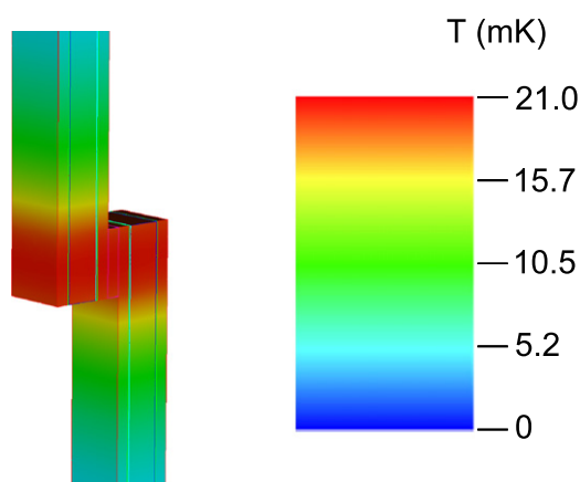
Figure 8. A three-dimensional visualisation of the temperature profile through a soldered joint which is operating at 77 K and conducts 100 A. The joint consists of a cuboid of Pb_{38}Sn_{62} solder, 20 \mu m thick with 4 mm \times 4 mm sides, between two multilayered REBCO superconducting tapes which each consist of Cu/Ag/Hastelloy/REBCO/Ag/Cu. The thicknesses of the layers are given in table 3. Heat conduction into the cryogen takes account of buoyancy or equivalently the direction of gravity which in this figure is taken to be in the long direction of the tapes, broadly down the page.
