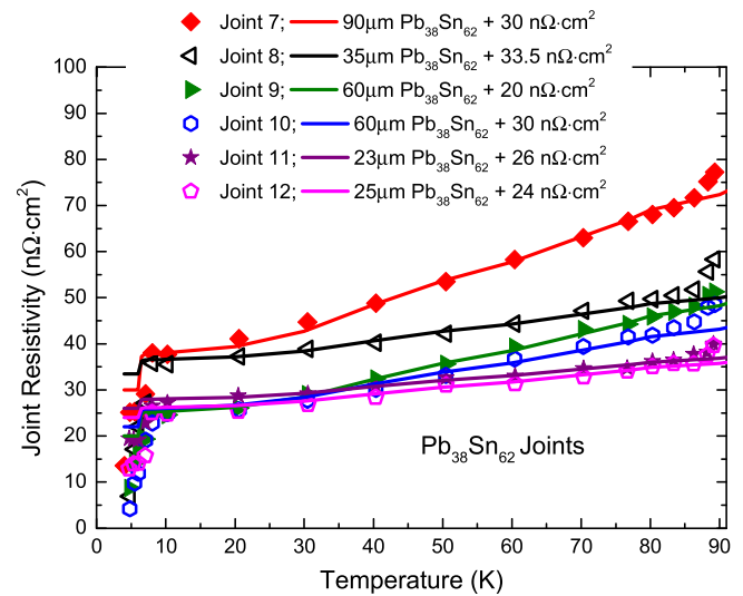
Figure 12. Joint resistivity as a function of temperature for six joints fabricated using \text{Pb}_{38}\text{Sn}_{62} solder. The soldered joint areas were 4\text{ mm} \times 3.3\text{ mm} , 4\text{ mm} \times 3.5\text{ mm} , 4\text{ mm} \times 3.8\text{ mm} , 4\text{ mm} \times 3.9\text{ mm} , 4\text{ mm} \times 3.6\text{ mm} and 4\text{ mm} \times 3.8\text{ mm} for joints 7–12 respectively. Lines are fits using equation (5.1) which uses the thickness of the solder and the interfacial resistivity as free parameters. The interfacial resistivity is also assumed to be temperature independent. Joints 11 and 12 were found to have an interfacial resistivity of 25\text{ n}\Omega\text{ cm}^2 . However, the resistivity of other joints cannot be described properly using equation (5.1) because the derived thicknesses of the solder (which microscopy shows in 25\text{ }\mu\text{m} ) are not physically large. Measurements were made in zero applied field.
