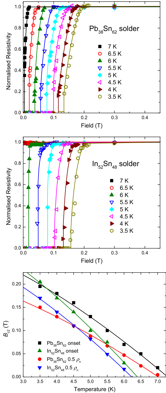
Figure 5. The normalised resistivity of \text{Pb}_{38}\text{Sn}_{62} (upper) and \text{In}_{52}\text{Sn}_{48} (middle) solders as a function of (increasing) applied magnetic fields at low temperatures. Lines are guide to the eye. Lower: upper critical field ( B_{c2} ) of \text{Pb}_{38}\text{Sn}_{62} and \text{In}_{52}\text{Sn}_{48} solders as a function of temperature. B_{c2} defined using two criteria: at the onset of transition (solid triangles and squares) and when the solder resistance equalled half of the normal state value (solid down triangles and circles). Curves are fitted using the W–H–H equation [75] and the derived parameters obtained are listed in table 6.
