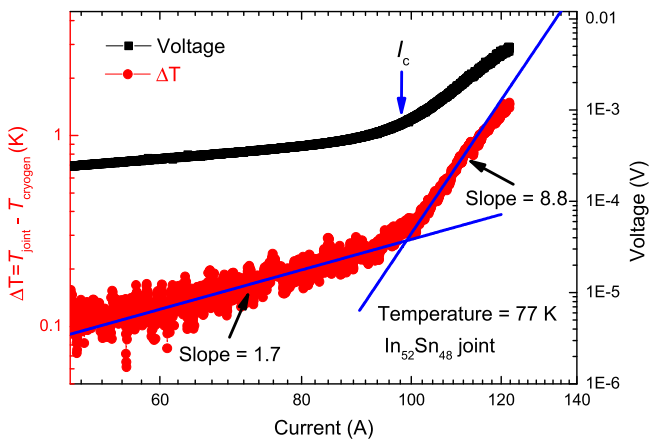
Figure 17. The voltage across a joint and the temperature difference between the centre of the joint and the cryogen, as a function of current through the joint. The joint consisted of two REBCO tapes joined by a cuboid of \text{In}_{52}\text{Sn}_{48} solder of joint area dimensions 4 \text{ mm} \times 4.8 \text{ mm} and thickness of 0.41 \text{ mm} . Measurements were made in zero applied field.
