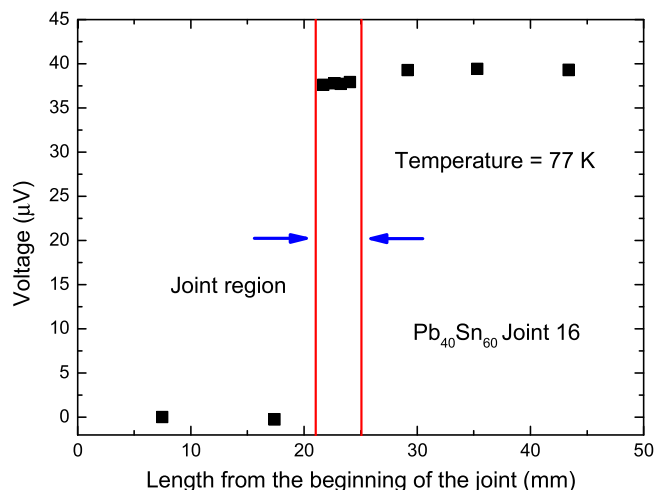
Figure 9. The voltage across a soldered joint at 77 K with respect to a tap about 21 mm from the joint on the grounded REBCO tape, when carrying 80 A. The joint consisted of two REBCO tapes joined by a cuboid of Pb_{40}Sn_{60} solder of joint area 4 mm \times 4 mm and nominal thickness of \sim 25 \mu m . Generic behaviour is observed where the voltage differences between two taps that are both on either one of the component REBCO tapes is zero but the total voltage across the joint is observed between any two taps that are on the different tapes.
