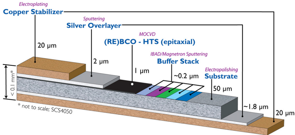
Figure 1. Multilayer structure of a SuperPower IBAD-MOCVD REBCO coated-conductor superconducting tape [40].
