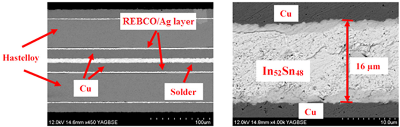
Figure 2. SEM images of a soldered joint made using two SuperPower REBCO tapes and \text{In}_{52}\text{Sn}_{48} solder between them.
