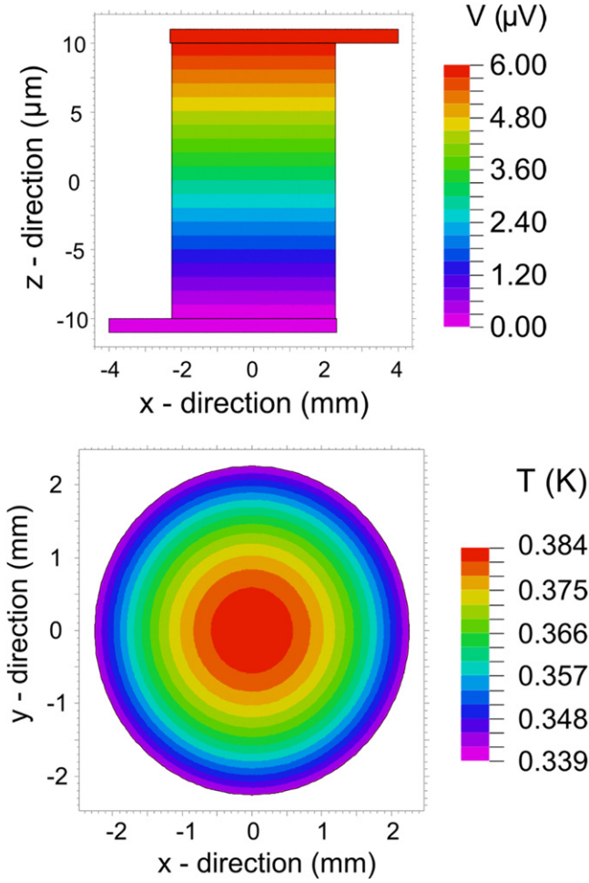
Figure 7. The voltage profile and temperature profile through an idealised soldered joint. The joint consists of a cylinder of solder, 20 \mu\text{m} thick with a radius of 4/\sqrt{\pi} mm, which connects two 1 \mu\text{m} thick, 4.6 mm wide, thermally insulating superconducting slabs. The voltage is generated by injecting 100 A into the top right-hand side of the upper superconducting slab which passes through the joint and flows to ground through the bottom superconducting slab. The solder has the properties of \text{Pb}_{38}\text{Sn}_{62} operating at 77 K. Upper: the voltage profile is a cutaway through the centre of the joint along its length. The gradient in the voltage (i.e. the electric field) is uniform within the solder (i.e. y = 0 ). Lower: The temperature profile is a slice through the centre of the joint (i.e. z = 0 ). The temperature gradient throughout the slice is radial. Heat conduction into the cryogen takes account of buoyancy or equivalently the direction of gravity which in this figure is down the axis of the solder.
