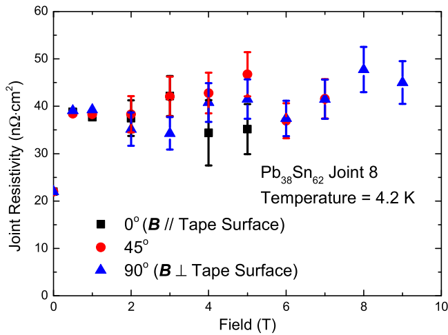
Figure 16. Joint resistivity of soldered joints at 4.2 K as a function of field at different orientations of the tape with respect to the applied field. The solder used was \text{Pb}_{38}\text{Sn}_{62} and the soldered joint area was 4 \text{ mm} \times 3.5 \text{ mm} and an expected nominal thickness of \sim 25 \mu\text{m} . The angles are those between the applied field and the surface of the tape.
