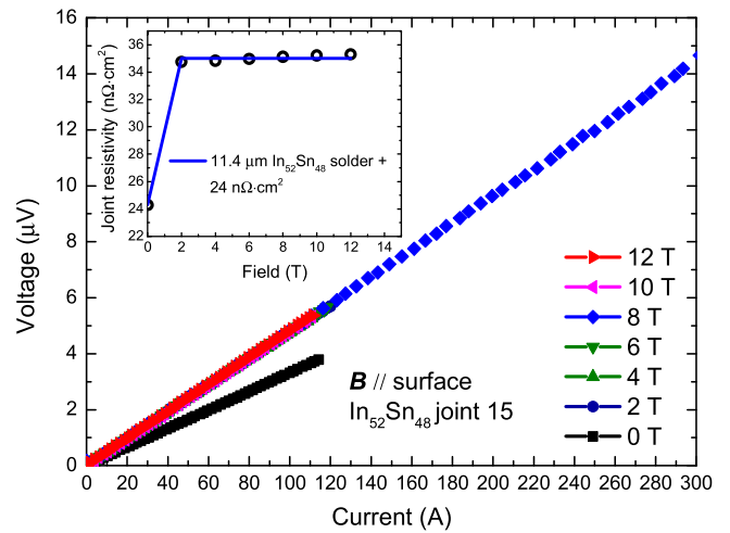
Figure 14. Voltage–current ( V – I ) traces at 4.2 K for a joint fabricated using \text{In}_{52}\text{Sn}_{48} solder as a function of the field applied parallel to the broad surface of the tape. Most V – I traces were taken up to 120 A, although data up to 300 A at 8 T are also shown. Inset: joint resistivity of the \text{In}_{52}\text{Sn}_{48} joint at 4.2 K as a function of applied field. The line is a fit using the assumption that joint resistivity is solely due to an 11.4\text{ }\mu\text{m} thick \text{In}_{52}\text{Sn}_{48} solder layer with a temperature independent interfacial resistivity of 24\text{ n}\Omega\text{ cm}^2 .
