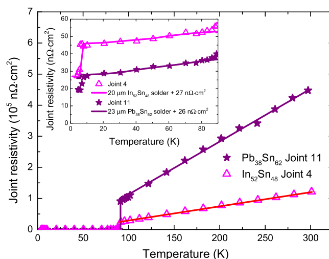
Figure 10. Joint resistivity as a function of temperature for two soldered joints made using In_{52}Sn_{48} and Pb_{38}Sn_{62} solders. The resistivity of the joints at 40 K were 47 n\Omega cm^2 (resistance \sim 300 n\Omega ) and 31 n\Omega cm^2 (resistance \sim 210 n\Omega ) for the In_{52}Sn_{48} and Pb_{38}Sn_{62} joints respectively. Measurements were made in zero applied field.
