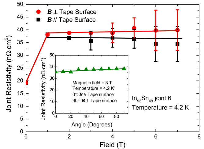
Figure 15. Magnetoresistance of the joint resistivity at 4.2 K as a function of applied magnetic field. The solder used was \text{In}_{52}\text{Sn}_{48} and the soldered joint area was 4\text{ mm} \times 18.6\text{ mm} and an expected nominal thickness of \sim 25\text{ }\mu\text{m} . Inset shows the joint resistivity as a function of the angle between the orientation of the tape and the direction of the applied field at 3 T and 4.2 K.
