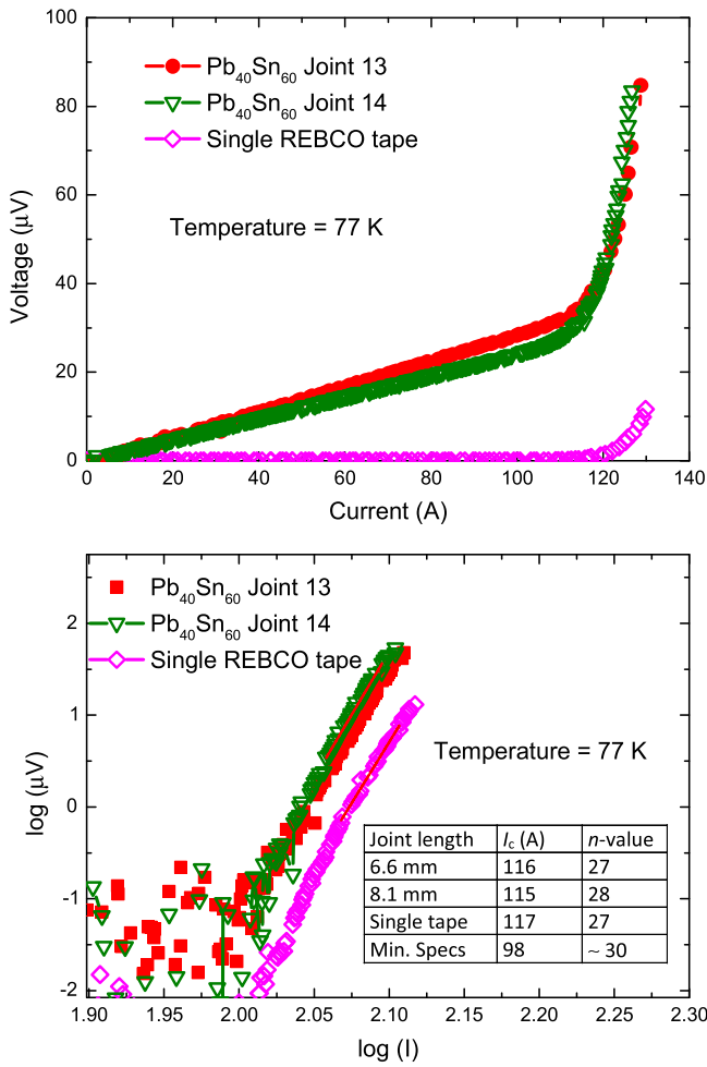
Figure 13. Voltage–current ( V – I ) traces for two soldered joints and a single REBCO tape. Upper: the raw V – I data. Lower: data replotted with the resistive contribution from the joints removed. For Joint 13 the solder used was \text{Pb}_{40}\text{Sn}_{60} and the soldered joint area was 4\text{ mm} \times 6.6\text{ mm} . For joint 14 the soldered joint area was 4\text{ mm} \times 8.1\text{ mm} . In both joints the expected nominal thickness was \sim 25\text{ }\mu\text{m} . The critical current and the n -value are similar in the two joints and the tape. Measurements were made in zero applied field.
