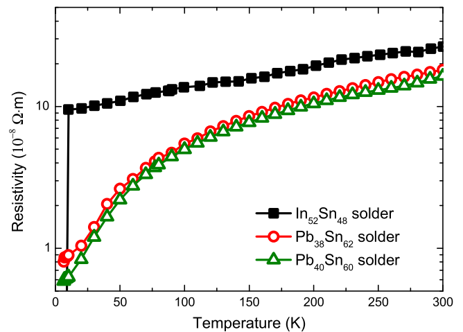
Figure 4. Resistivity as a function of temperature for \text{In}_{52}\text{Sn}_{48} , \text{Pb}_{38}\text{Sn}_{62} and \text{Pb}_{40}\text{Sn}_{60} solders at temperatures below 300 K. \text{In}_{52}\text{Sn}_{48} and \text{Pb}_{38}\text{Sn}_{62} were fabricated in Durham and \text{Pb}_{40}\text{Sn}_{60} was purchased from a commercial supplier.
