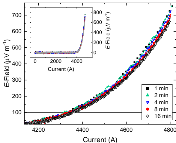
Fig. 4: Core I_c traces using different trace times, without the nano-amplifier, showing trace time dependency.
