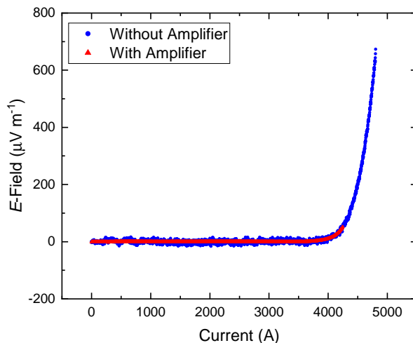
Fig. 3: 8 minute I_c traces for the core, with the nano-amplifier (in red) and without the nano-amplifier (in blue).
