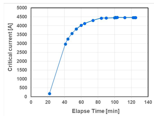
Fig. 4. Observed critical current of the cable core as a function of the time after immersing the cable in liquid nitrogen bath.
