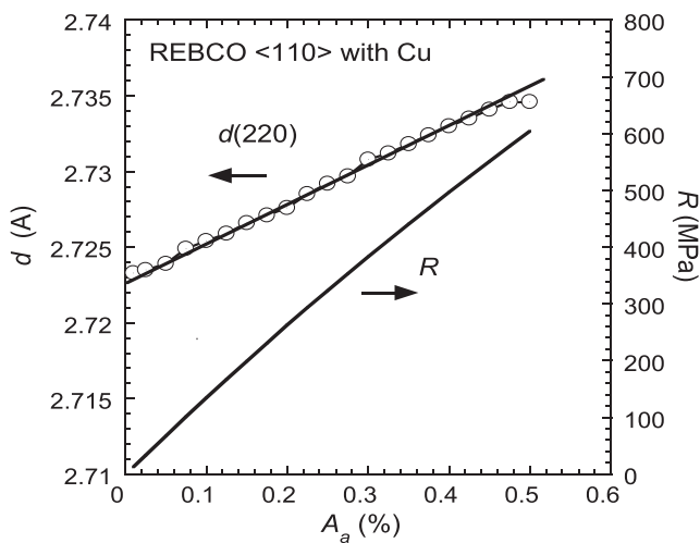
FIG. 12. Applied tensile strain dependence of lattice spacing d(220) together with the stress – strain curve for REBCO \langle 110 \rangle with Cu.
