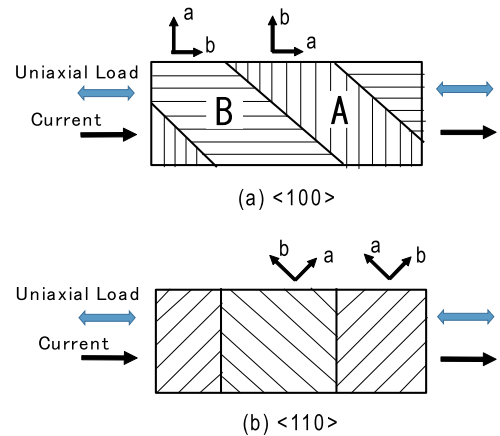
FIG. 14. \langle 100 \rangle (a) and \langle 110 \rangle (b) oriented twin structures along the tape axis.
