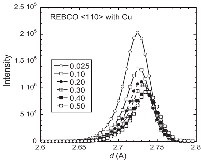
FIG. 11. Diffraction profiles due to (220) plane of \text{REBa}_2\text{Cu}_3\text{O}_{8+x} phase during the increase of applied tensile strain for REBCO \langle 110 \rangle with Cu.
