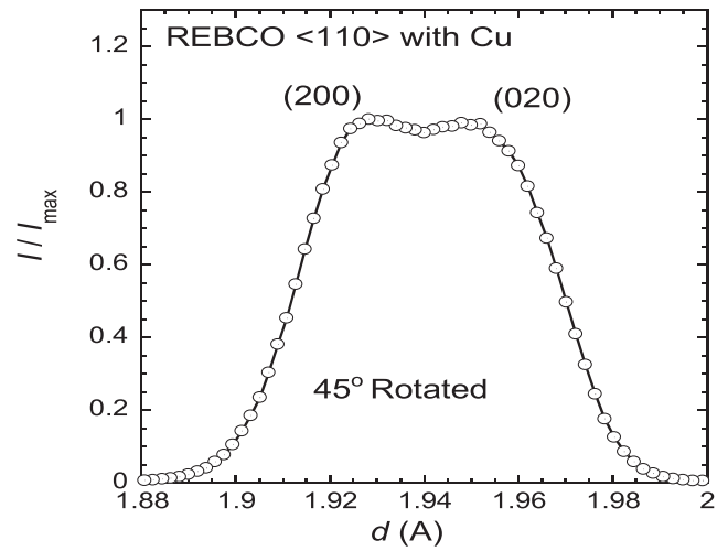
FIG. 13. Diffraction pattern of (200) and (020) lattice planes at the 45 degrees rotated position from the scattering vector axis for REBCO \langle 110 \rangle with Cu.
