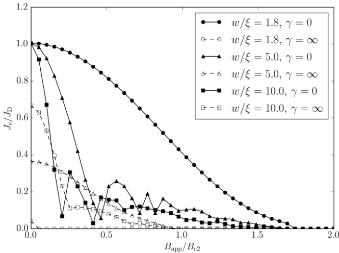
Fig. 4. Critical current density J_c against mean external magnetic field B_{\text{app}} for a superconducting system with \kappa = 10, \eta = 1 and l = 60\xi for varying width w . J_c and B_{\text{app}} are expressed in units of the depairing current J_D and the upper critical field B_{c2} for each superconductor respectively. The critical current was determined using Ekin's offset method using a critical electric field E_c = 0.01\phi_0/2\pi\xi\tau and extrapolating to \langle E_x \rangle = 0 .
