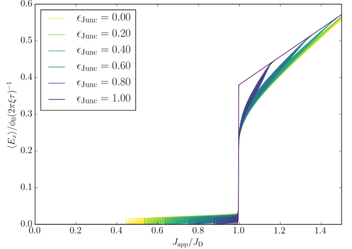
Fig. 6. Average electric field \langle E_x \rangle against external applied current J_{\text{app}} for a superconducting film containing a 2\xi wide 'junction' region in its centre, in which the local T_c term \epsilon_{\text{junc}} is variable. The surrounding superconducting domain was parameterised with \eta = 1, \kappa = 10 and dimensions w = 20\xi and l = 60\xi , with periodic boundary conditions applied in the x -direction and insulating boundary conditions applied in the y -direction. At each external magnetic field, the system was first initialised in the bulk Meissner state and the external magnetic field B_{\text{app}} was raised to the desired value. The external current density J_{\text{app}} was then slowly swept up to above the depairing current J_D .
