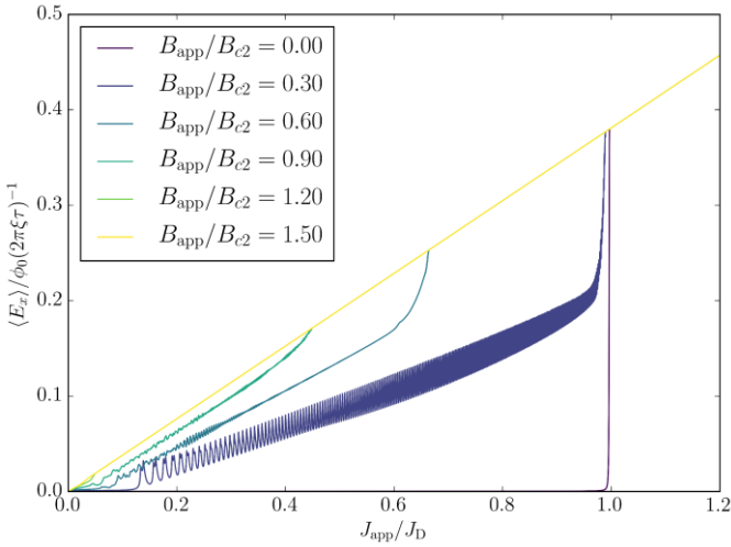
Fig. 3. Average electric field \langle E_x \rangle against external applied current J_{\text{app}} for a superconducting film with w = 20\xi, l = 60\xi, \eta = 1 and \kappa = 10 subject to various external magnetic fields. Periodic boundary conditions were applied in the x -direction and insulating boundary conditions were applied in the y -direction. Systems were first initialised in the bulk Meissner state and the external magnetic field B_{\text{app}} was raised to the desired value. The external current density J_{\text{app}} was then slowly swept up to above the depairing current J_D .
