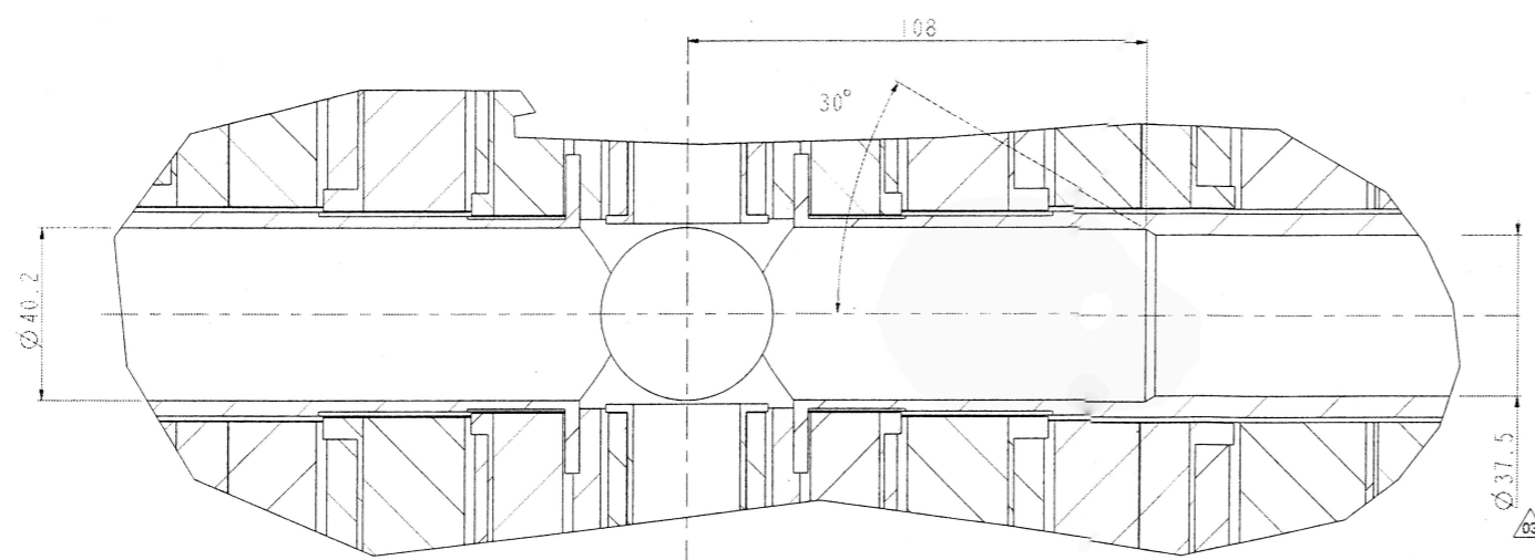
SAMPLE SPACE DETAILS DETAIL X SCALE 1:1
