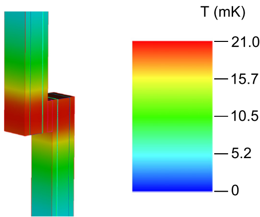
Figure 8. A three-dimensional visualisation of the temperature profile through a soldered joint which is operating at 77 K and conducts 100 A. The joint consists of a cuboid of \text{Pb}_{38}\text{Sn}_{62} solder, 20 \mu\text{m} thick with 4 \text{ mm} \times 4 \text{ mm} sides, between two multilayered REBCO superconducting tapes which each consist of Cu/Ag/Hastelloy/REBCO/Ag/Cu. The thicknesses of the layers are given in table 3. Heat conduction into the cryogen takes account of buoyancy or equivalently the direction of gravity which in this figure is taken to be in the long direction of the tapes, broadly down the page.
