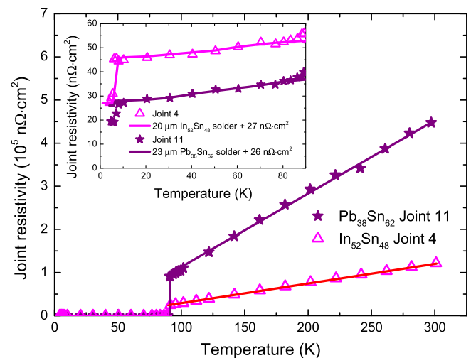
Figure 10. Joint resistivity as a function of temperature for two soldered joints made using \text{In}_{52}\text{Sn}_{48} and \text{Pb}_{38}\text{Sn}_{62} solders. The resistivity of the joints at 40 K were 47 \text{ n}\Omega \text{ cm}^2 (resistance \sim 300 \text{ n}\Omega ) and 31 \text{ n}\Omega \text{ cm}^2 (resistance \sim 210 \text{ n}\Omega ) for the \text{In}_{52}\text{Sn}_{48} and \text{Pb}_{38}\text{Sn}_{62} joints respectively. Measurements were made in zero applied field.
