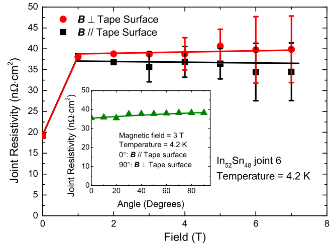
Figure 15. Magnetoresistance of the joint resistivity at 4.2 K as a function of applied magnetic field. The solder used was \text{In}_{52}\text{Sn}_{48} and the soldered joint area was 4 \text{ mm} \times 18.6 \text{ mm} and an expected nominal thickness of \sim 25 \mu\text{m} . Inset shows the joint resistivity as a function of the angle between the orientation of the tape and the direction of the applied field at 3 T and 4.2 K.
