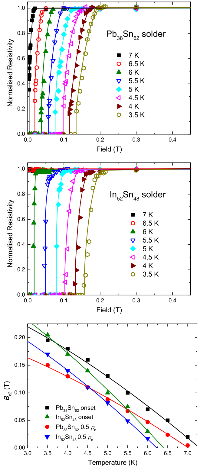
Figure 5. The normalised resistivity of Pb 38 Sn 62 (upper) and In 52 Sn 48 (middle) solders as a function of (increasing) applied magnetic fields at low temperatures. Lines are guide to the eye. Lower: upper critical field ( B_{c2} ) of Pb 38 Sn 62 and In 52 Sn 48 solders as a function of temperature. B_{c2} defined using two criteria: at the onset of transition (solid triangles and squares) and when the solder resistance equalled half of the normal state value (solid down triangles and circles). Curves are fitted using the W-H-H equation [75] and the derived parameters obtained are listed in table 6.
